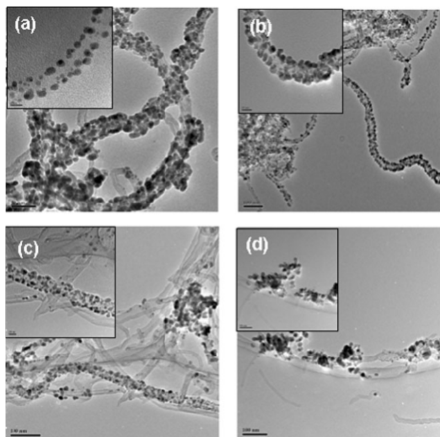
Fig. 1 TEM images of (a) Pd/IL- f -MWCNT 2a (scale bar: 50 nm, 10 nm for inset); (b) Pd/IL- f -MWCNT 2c prepared by anion exchange of 2a with NaSbF 6 (scale bar: 100 nm, 20 nm for inset); (c) Pd/IL- f -MWCNT 2c after 50 runs (scale bar: 100 nm, 20 nm for inset); (d) Pd/IL- f -MWCNT 2c after the 51st run (scale bar: 100 nm, 50 nm for inset).
